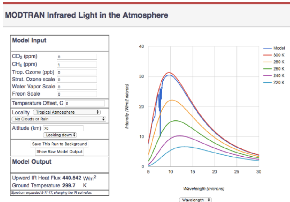
Figure 1: https://climatemodels.uchicago.edu/modtran/
